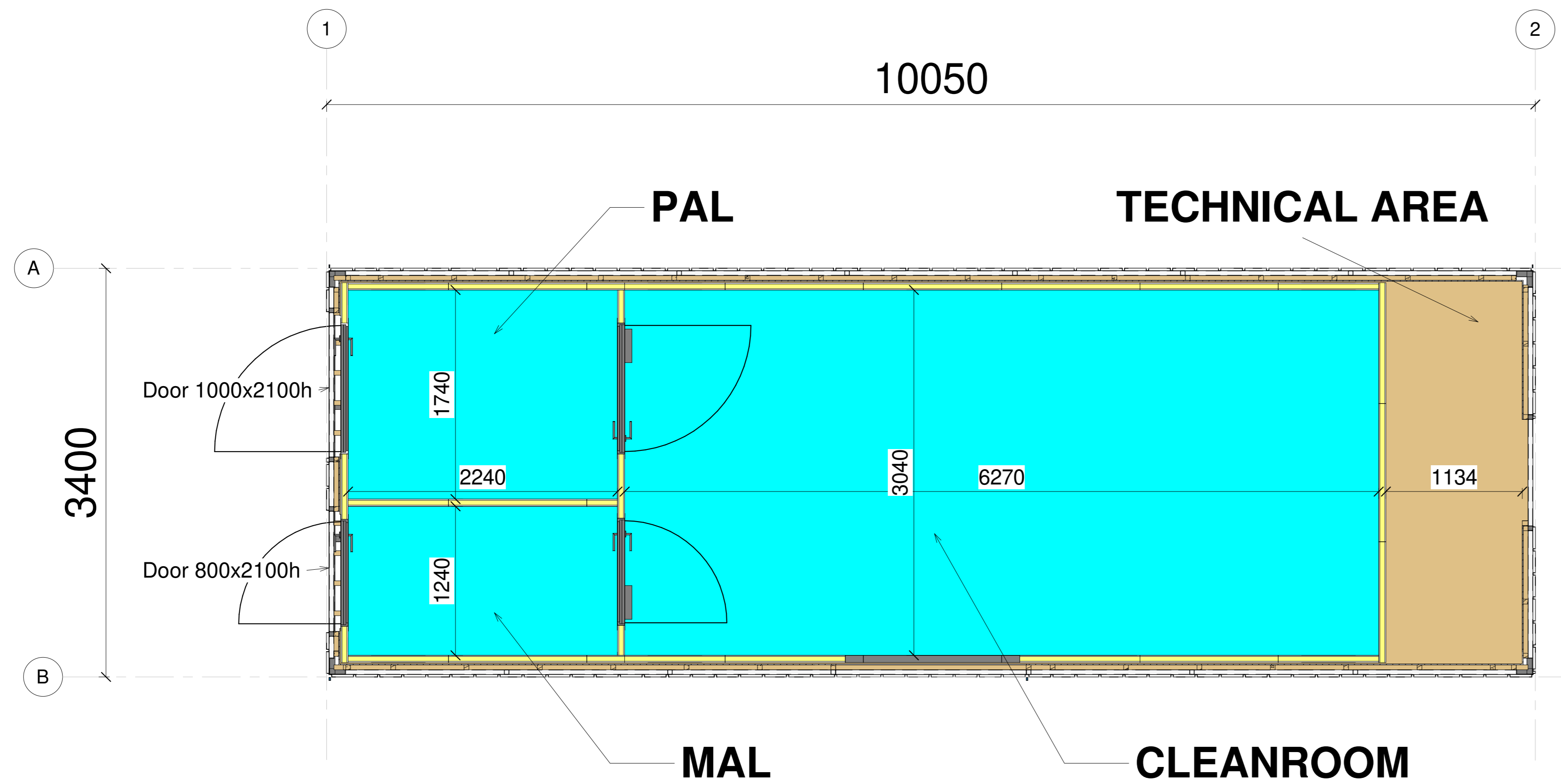
1 Level 1 1:25
